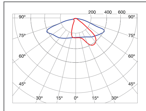
Indus (f) AB1 Vertical — Horizontal —
