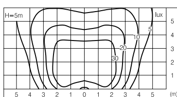
PHOTOMETRY Distribution: Asymmetric
