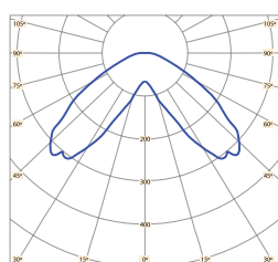
AL360 / 45° Lamp: 8 LED Modules
