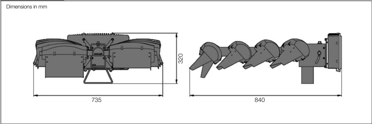
WS2006RS on 15m mast
