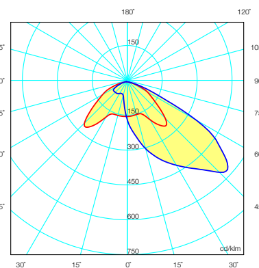
(202) Suitable for wide roadways and parking spaces with smaller distances between columns
