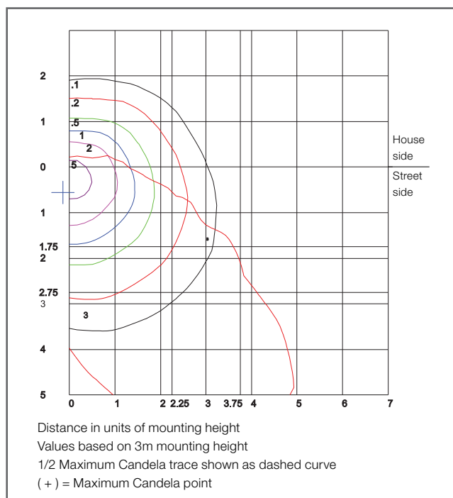
Polar diagram
