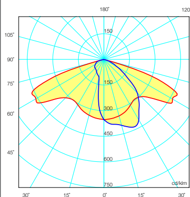
(010) Suitable for parking spaces and pedestrian crossings
