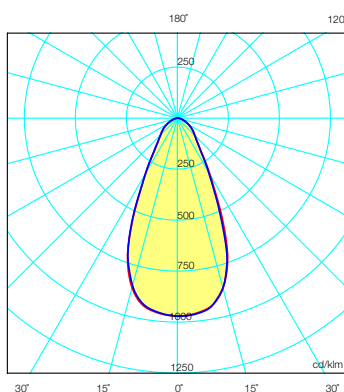
(100) Suitable for parking spaces and small distance between poles
