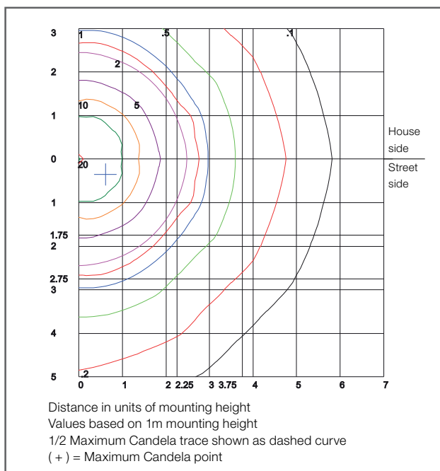
Polar diagram
