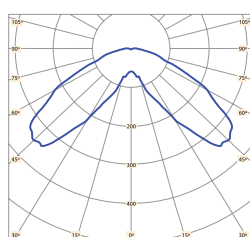
AL360 / 50° Lamp: 8 LED Modules
