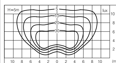
PHOTOMETRY Distribution: Batwing
