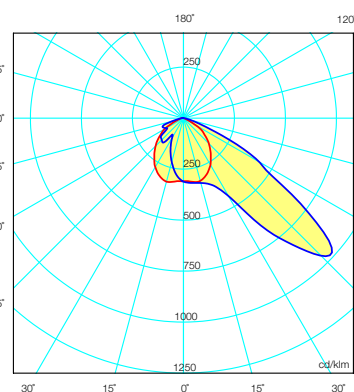
(101) Suitable for larger distance between poles and high mounting installations. Higher uniformity factor
