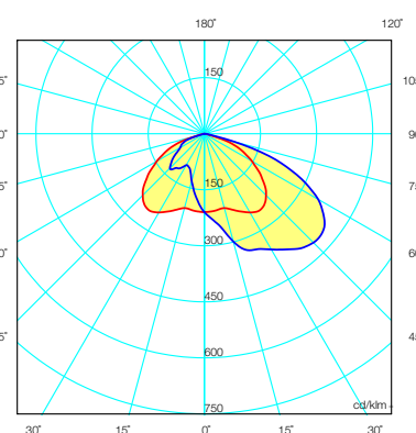
(110) Suitable for wide roadways, parking spaces. Smaller distance between columns
