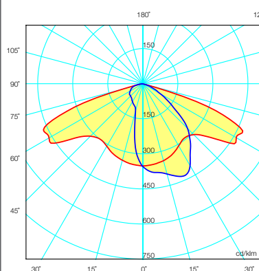
(010) Suitable for larger distance between poles and high mounting installations. Higher uniformity factor
