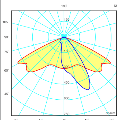
(000) Suitable for larger distance between poles and high mounting installations
