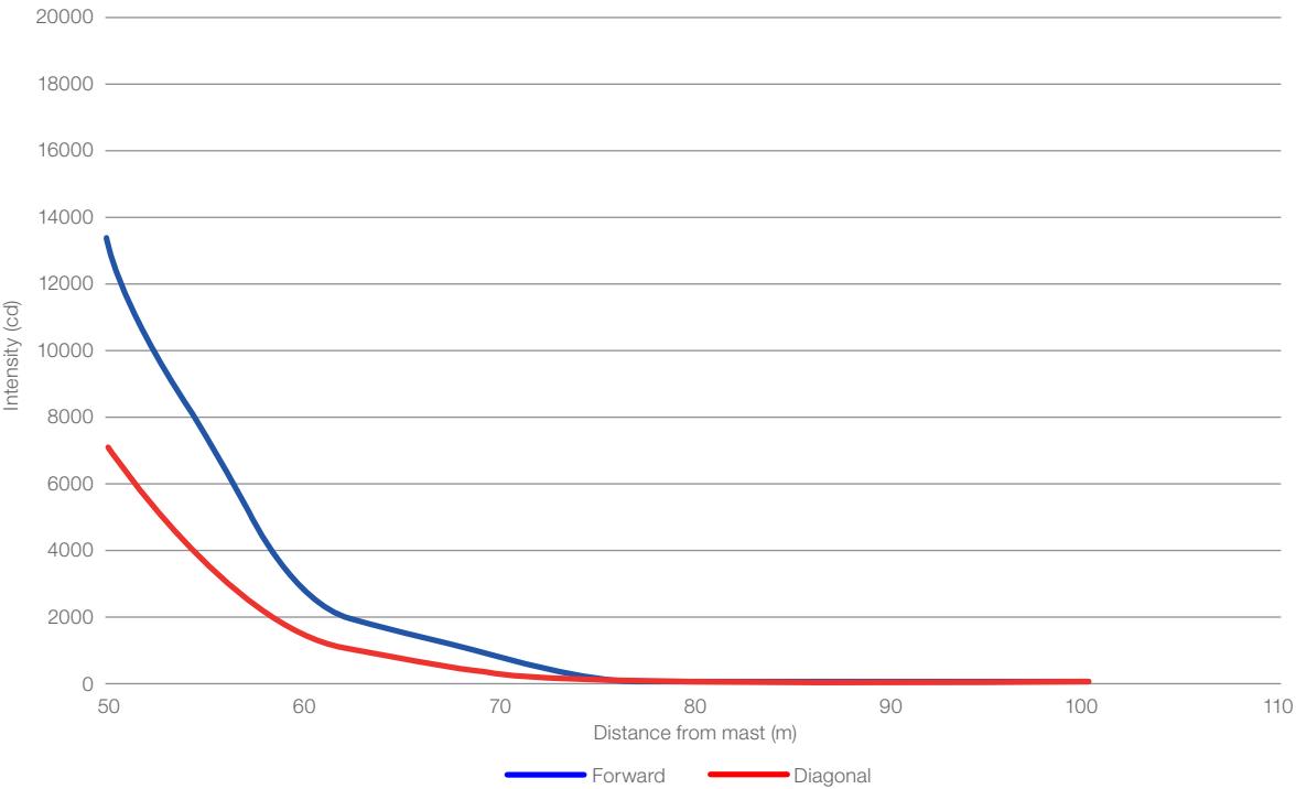
WS2006RS on 15m mast
