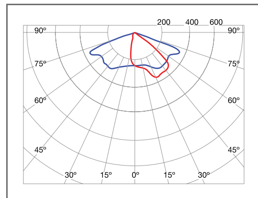
Indus (f) B1 Vertical — Horizontal —
