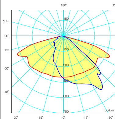
(020) Suitable for wide roadways, larger distance between columns
