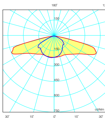
(200) Suitable for larger distance between columns, within bicycle paths
